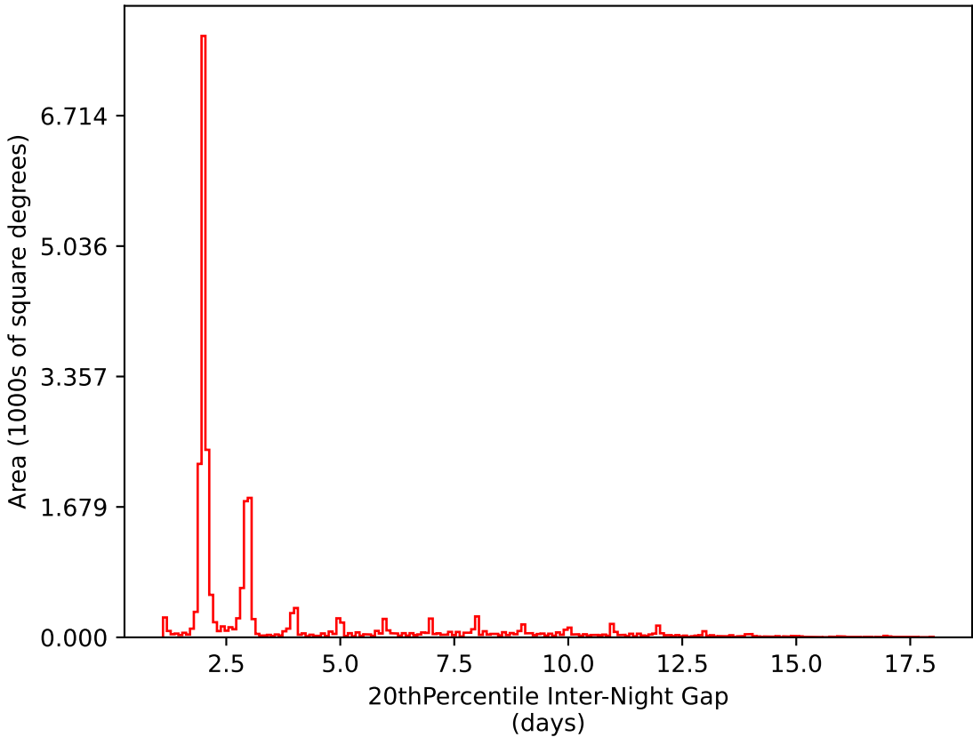
weather_cloudso35v3.4_10yrs All sky i band: 20thPercentile Inter-Night Gap
