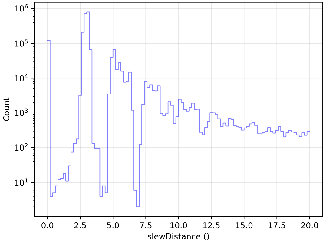
weather_cloudso35v3.4_10yrs All visits: Zoom Slew Distance Histogram
