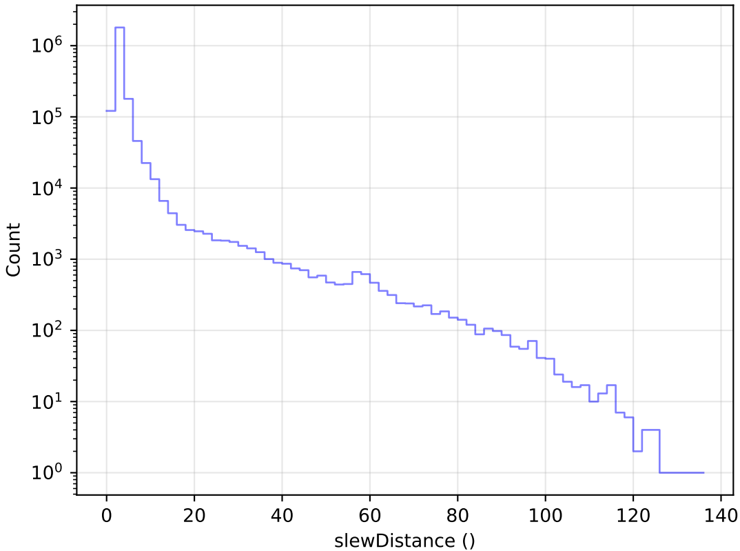
weather_cloudso35v3.4_10yrs All visits: Slew Distance Histogram
