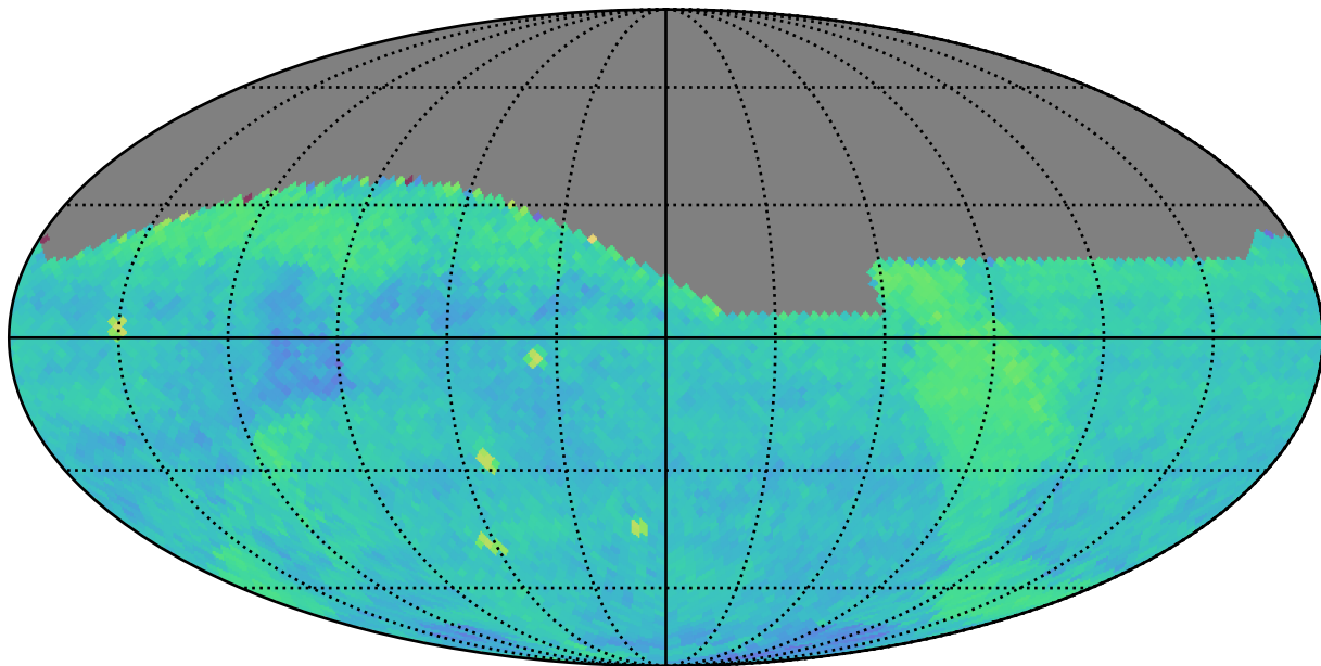
weather_cloudso35v3.4_10yrs (g or r or i): PairFraction
