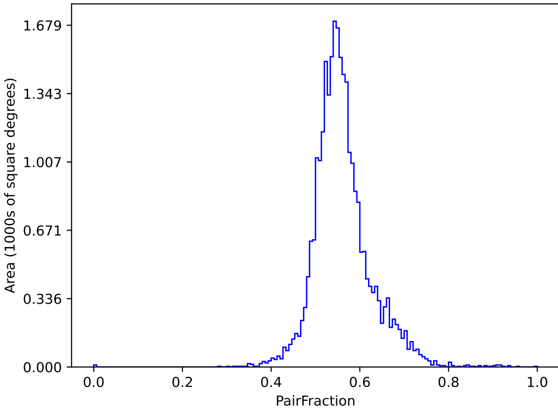
weather_cloudso35v3.4_10yrs (g or r or i): PairFraction
