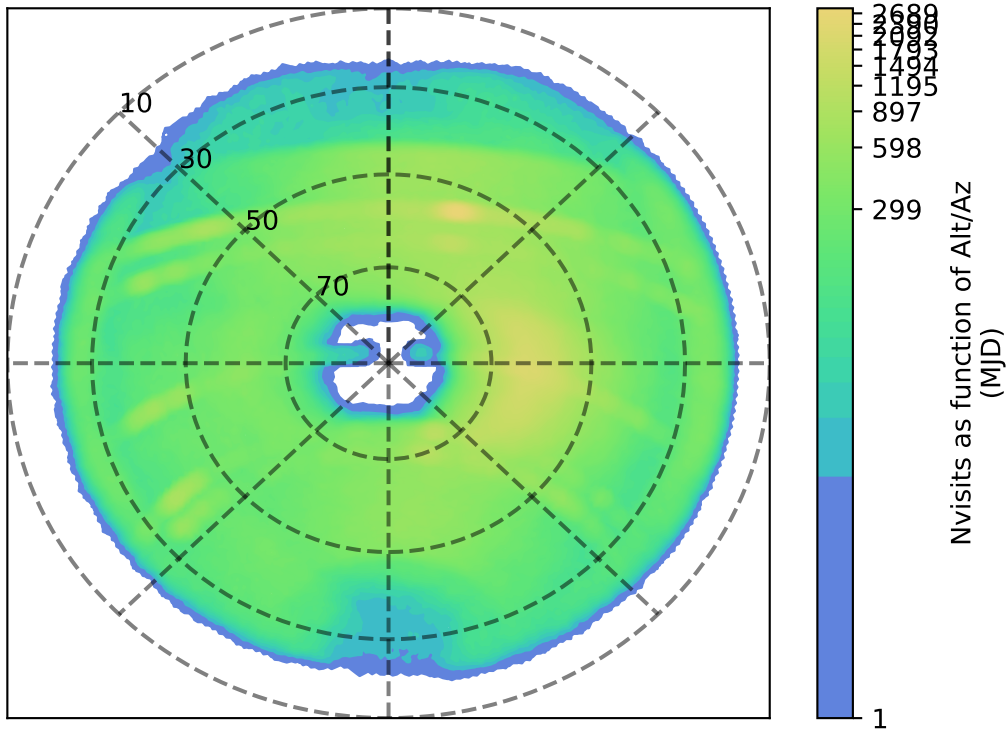
weather_cloudso35v3.4_10yrs z: Nvisits as function of Alt/Az
