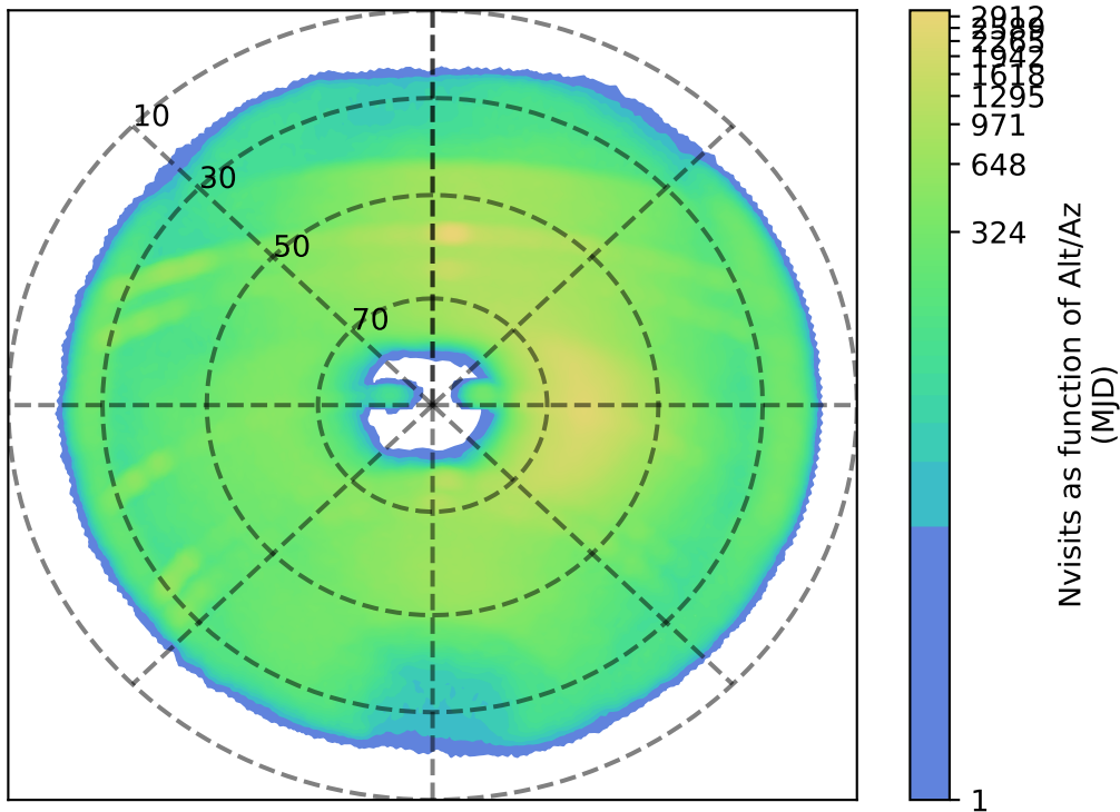
weather_cloudso35v3.4_10yrs i: Nvisits as function of Alt/Az
