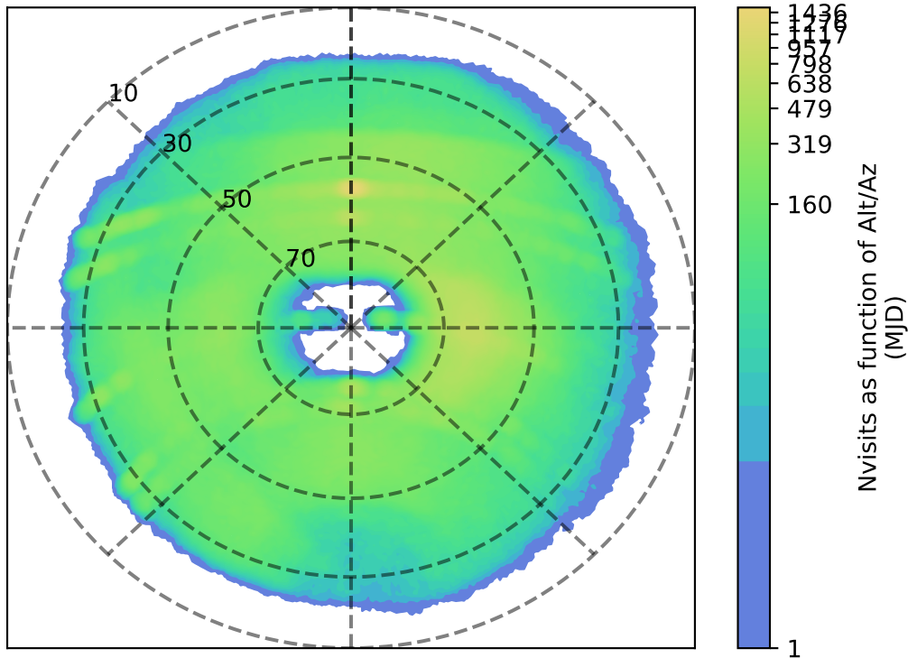
weather_cloudso35v3.4_10yrs g: Nvisits as function of Alt/Az
