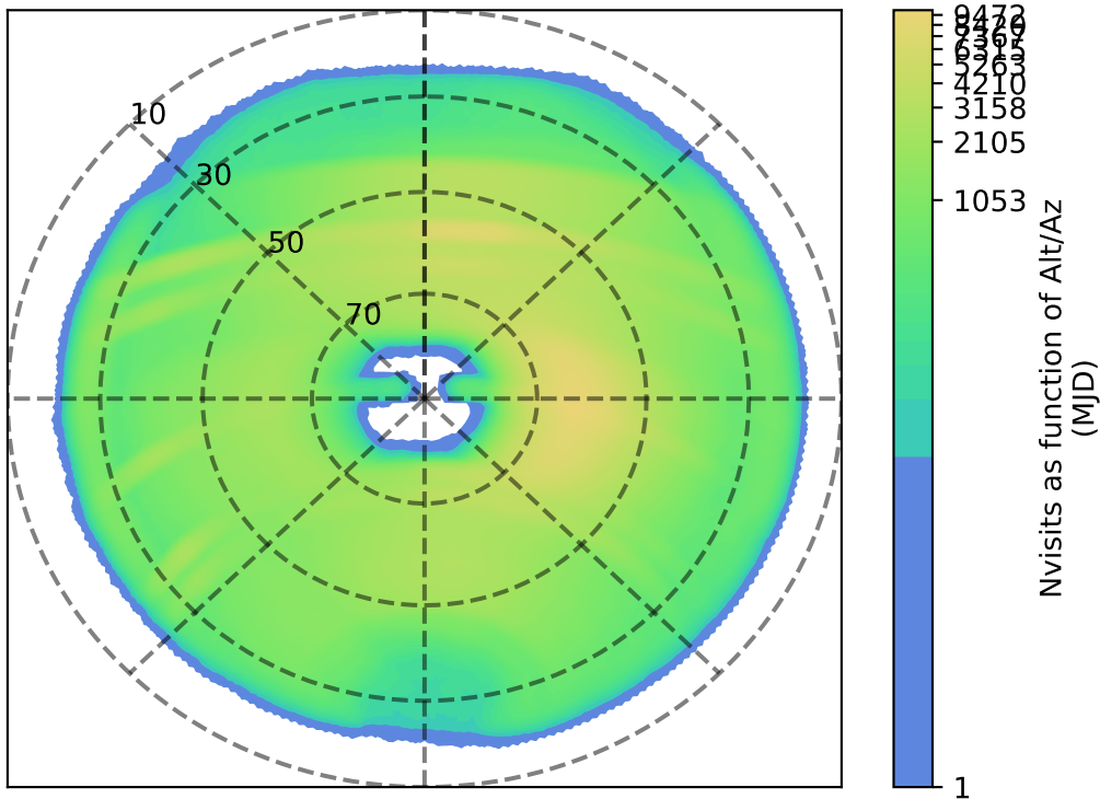
weather_cloudso35v3.4_10yrs : Nvisits as function of Alt/Az
