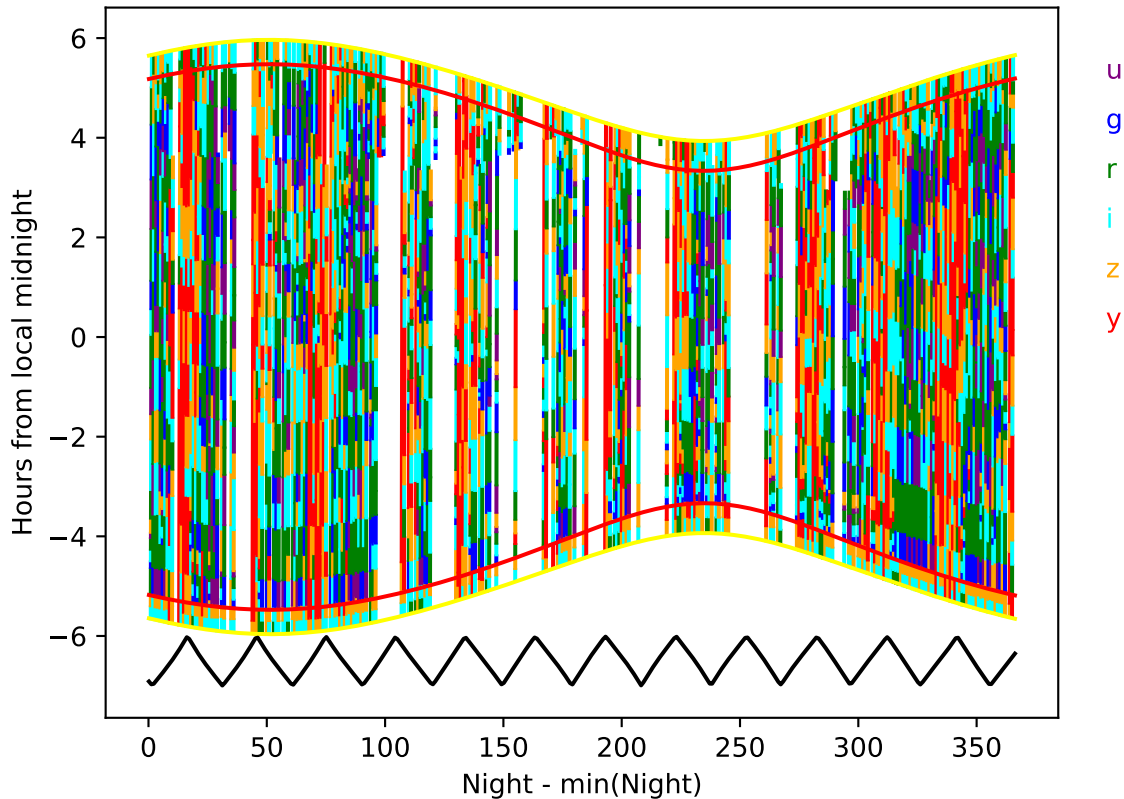
weather_cloudso35v3.4_10yrs year 5-6: Hourglass
