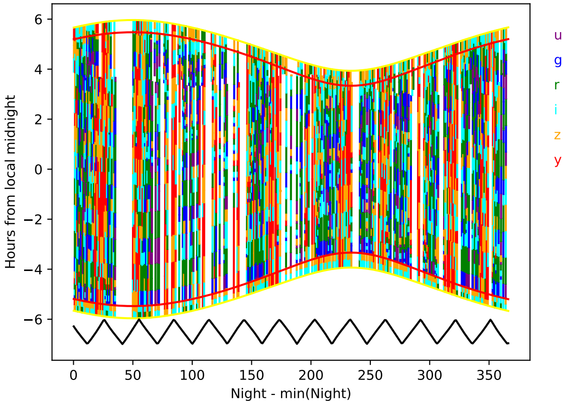
weather_cloudso35v3.4_10yrs year 4-5: Hourglass
