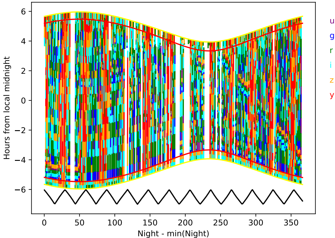
weather_cloudso35v3.4_10yrs year 1-2: Hourglass
