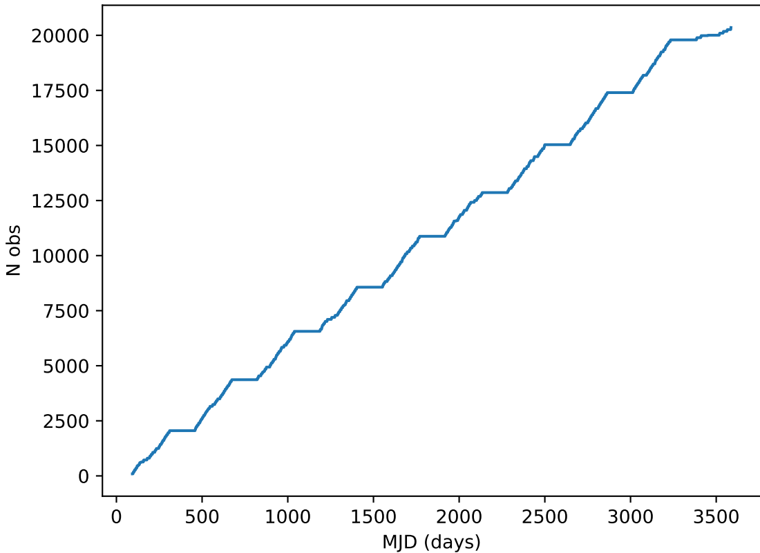
weather_cloudso35v3.4_10yrs note like DD:ECDFS%: Cumulative
