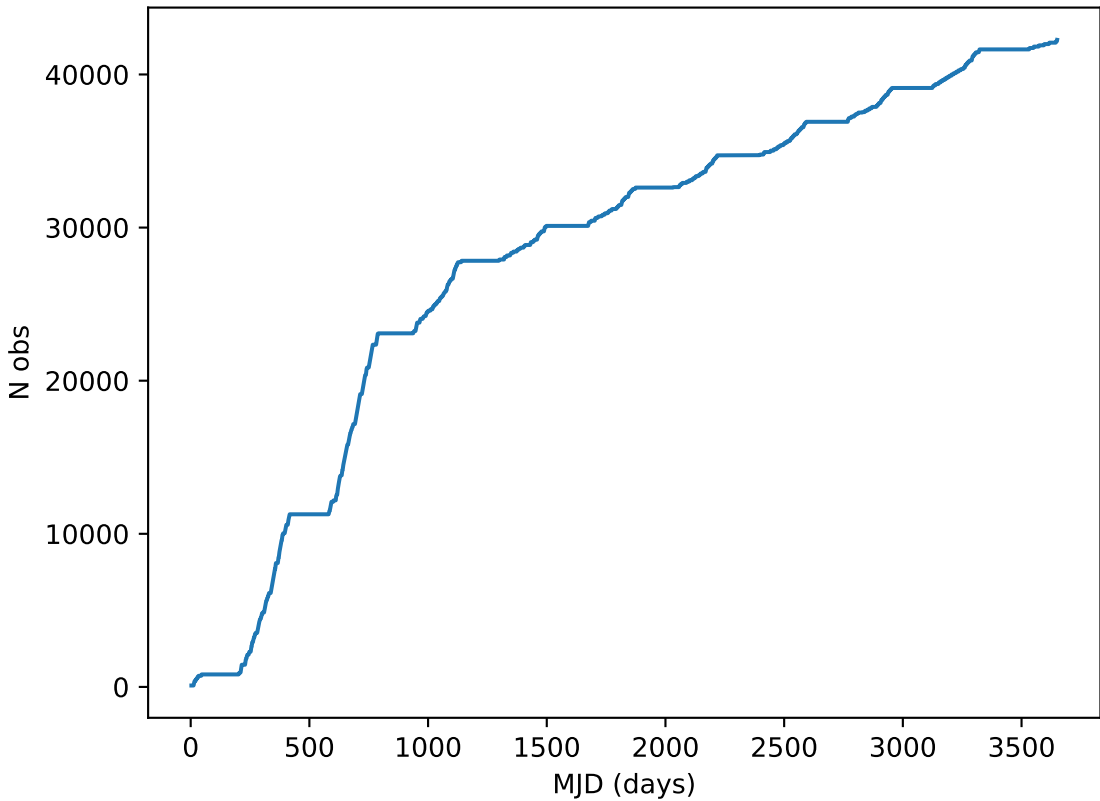
weather_cloudso35v3.4_10yrs note like DD:COSMOS%: Cumulative
