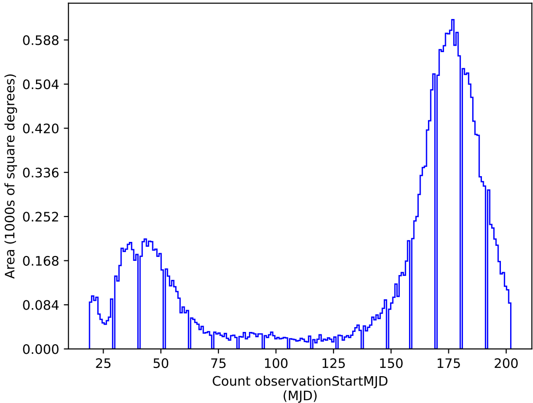
weather_cloudso35v3.4_10yrs z: Count observationStartMJD
