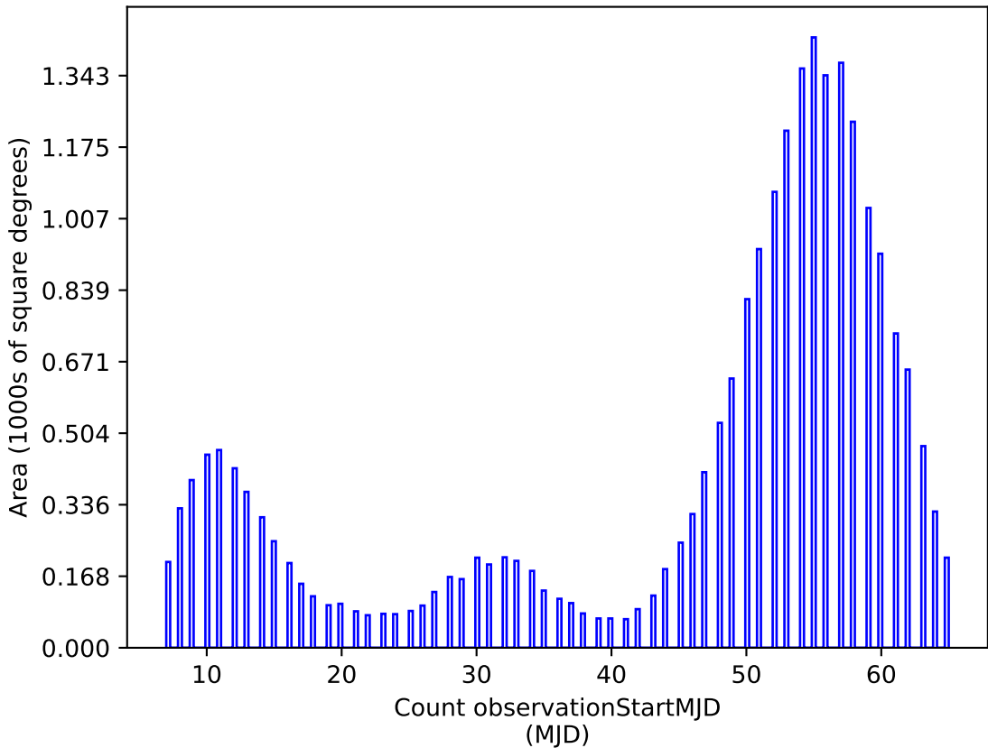
weather_cloudso35v3.4_10yrs u: Count observationStartMJD
