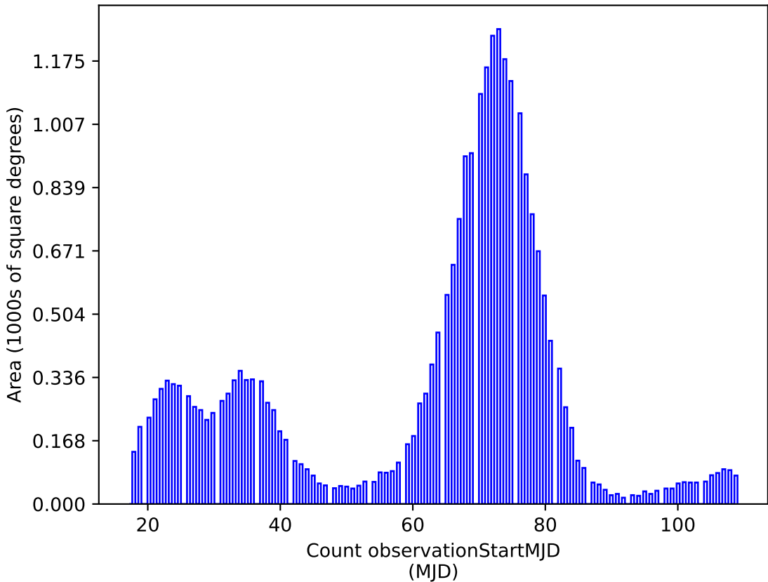
weather_cloudso35v3.4_10yrs g: Count observationStartMJD
