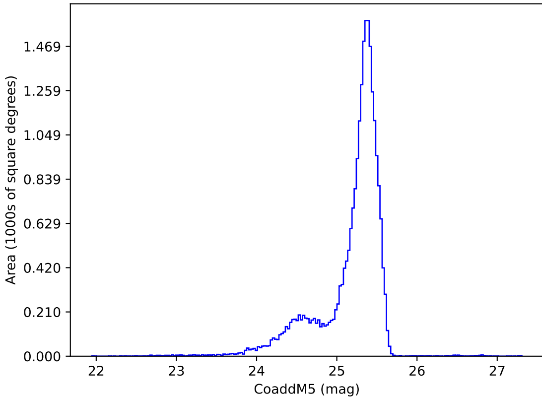
weather_cloudso35v3.4_10yrs u: CoaddM5
