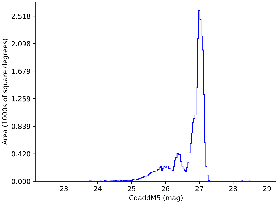
weather_cloudso35v3.4_10yrs r: CoaddM5
