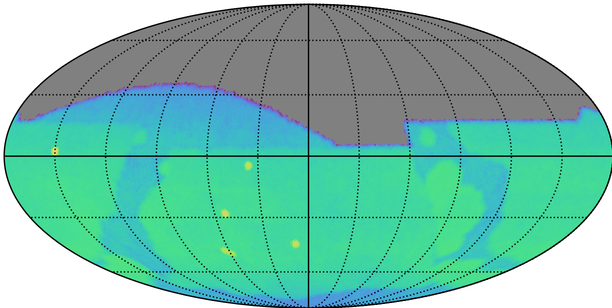
weather_cloudso35v3.4_10yrs g: CoaddM5
