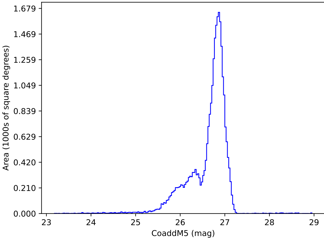
weather_cloudso35v3.4_10yrs g: CoaddM5
