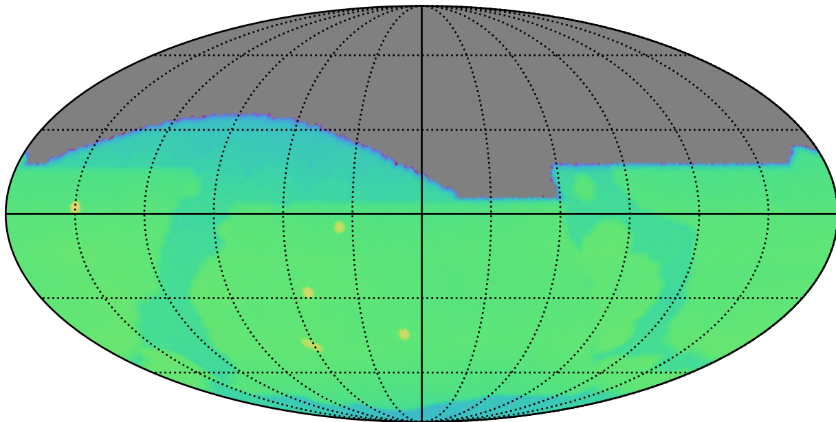
weather_cloudso35v3.4_10yrs : CoaddM5
