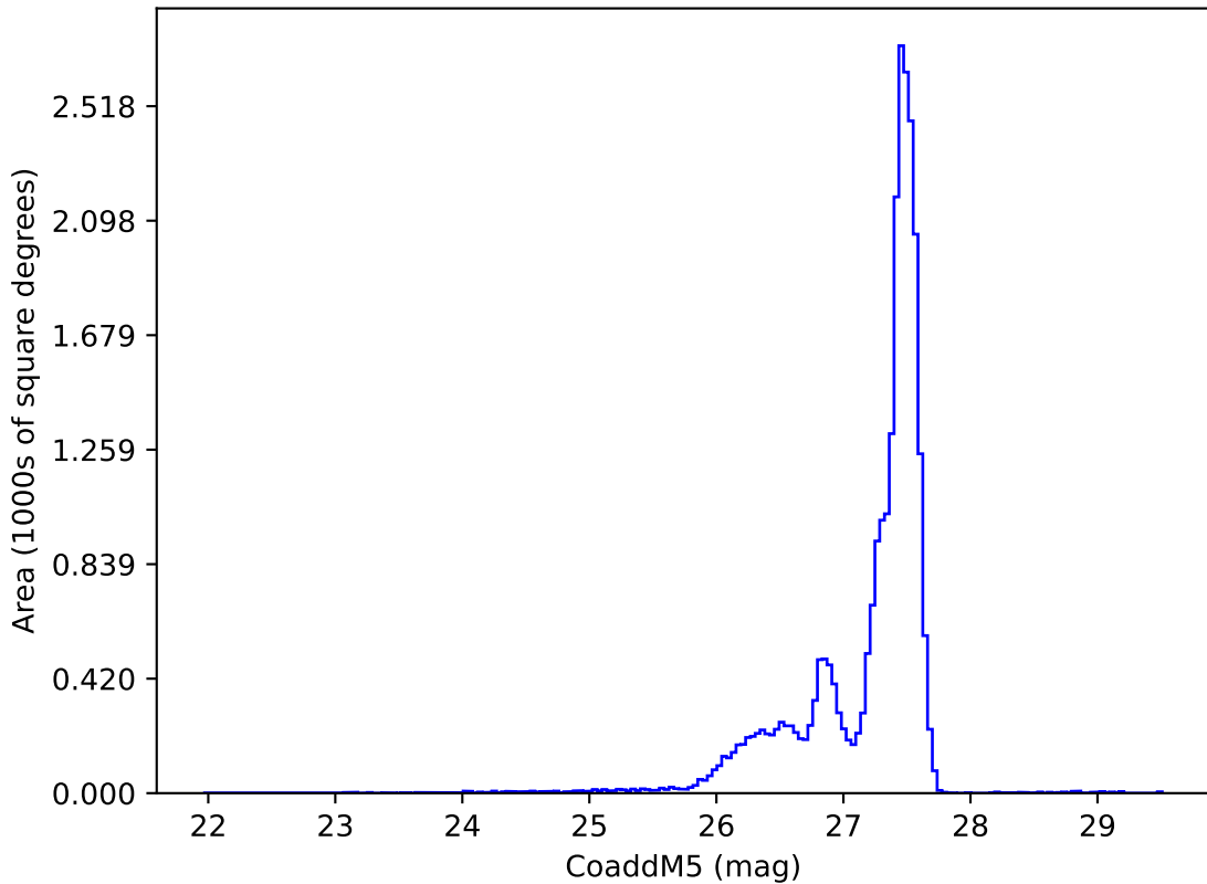
weather_cloudso35v3.4_10yrs : CoaddM5
