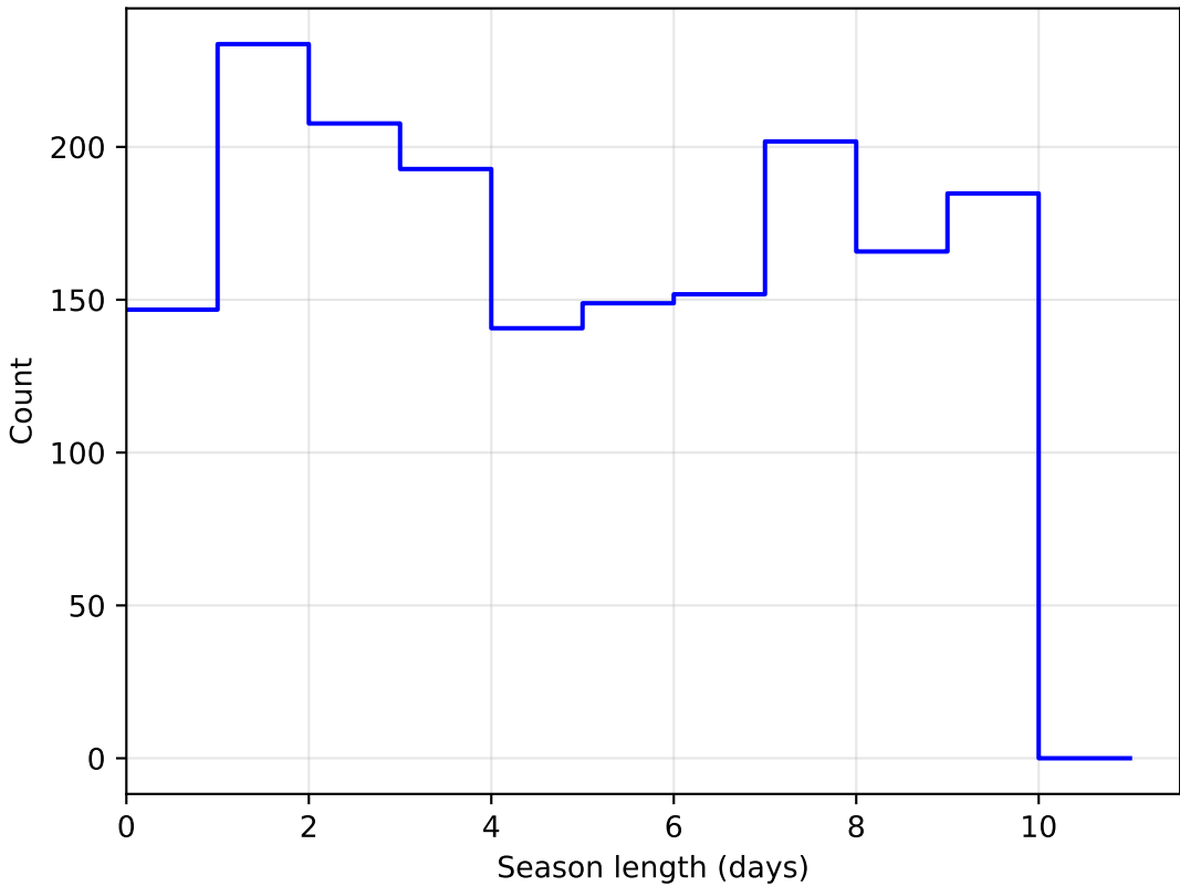
weather_cloudso35v3.4_10yrs DD:WFD all bands: SeasonLength
