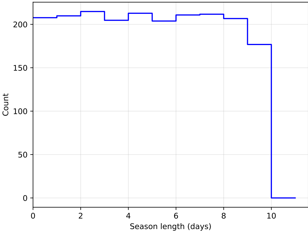
weather_cloudso35v3.4_10yrs DD:EDFS all bands: SeasonLength
