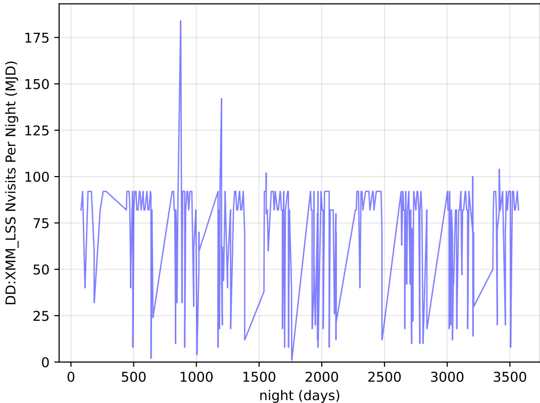
weather_cloudso35v3.4_10yrs all bands: DD:XMM_LSS Nvisits Per Night
