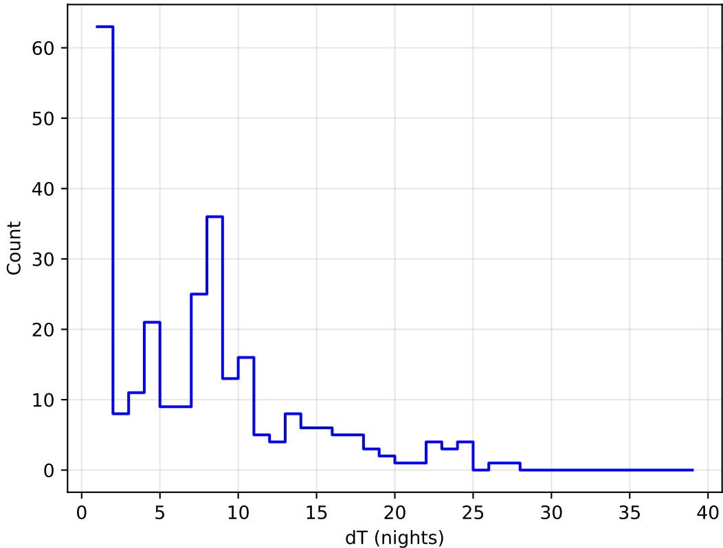
weather_cloudso35v3.4_10yrs all bands: DD:XMM_LSS Delta Nights Histogram
