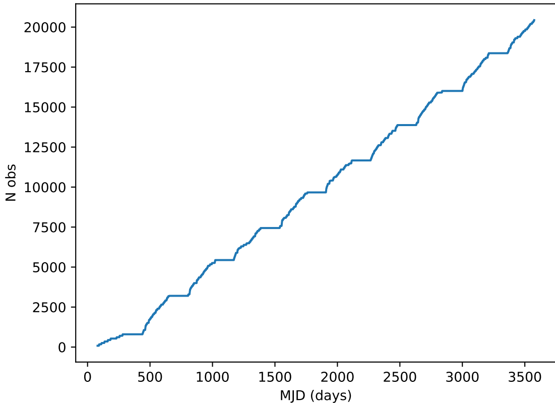
weather_cloudso35v3.4_10yrs all bands: DD:XMM_LSS Cumulative NVisits
