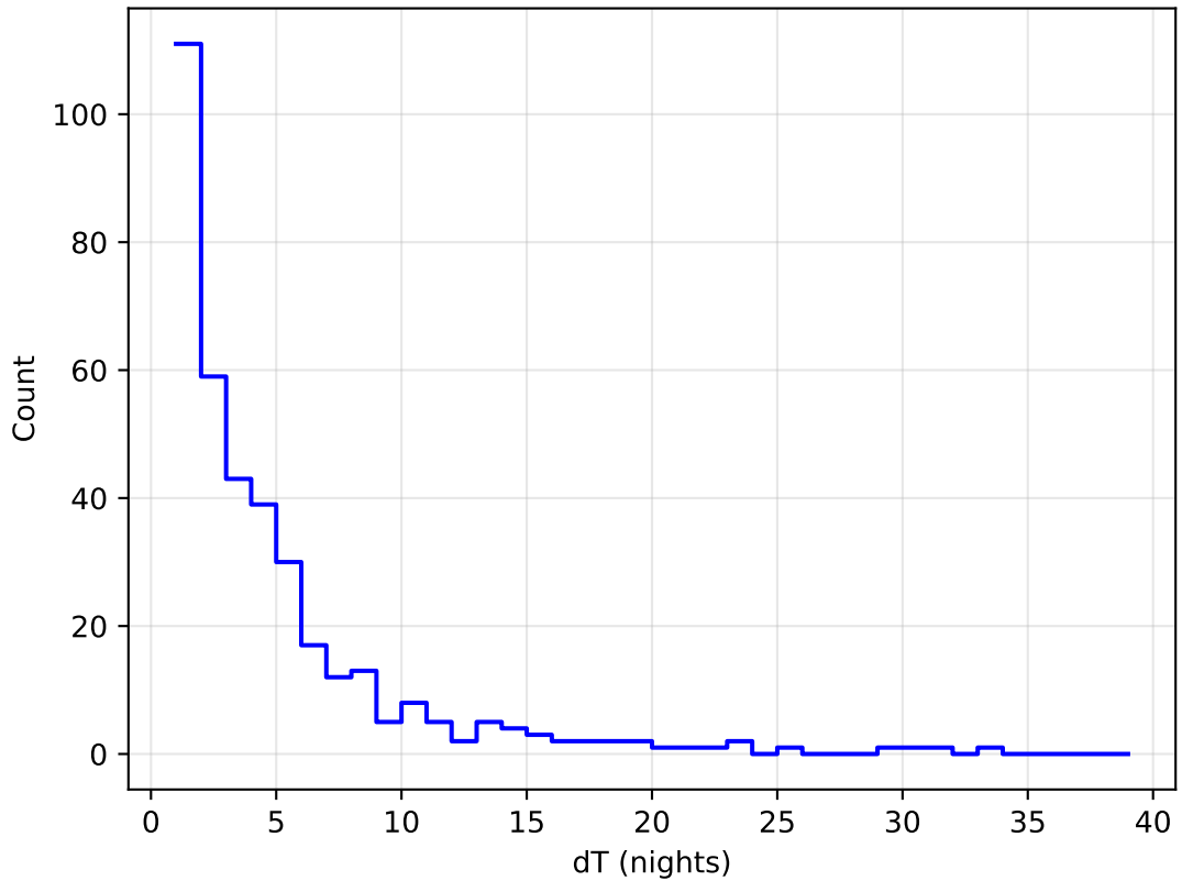
weather_cloudso35v3.4_10yrs all bands: DD:WFD Delta Nights Histogram
