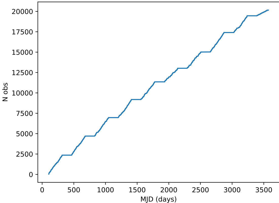
weather_cloudso35v3.4_10yrs all bands: DD:EDFS Cumulative NVisits
