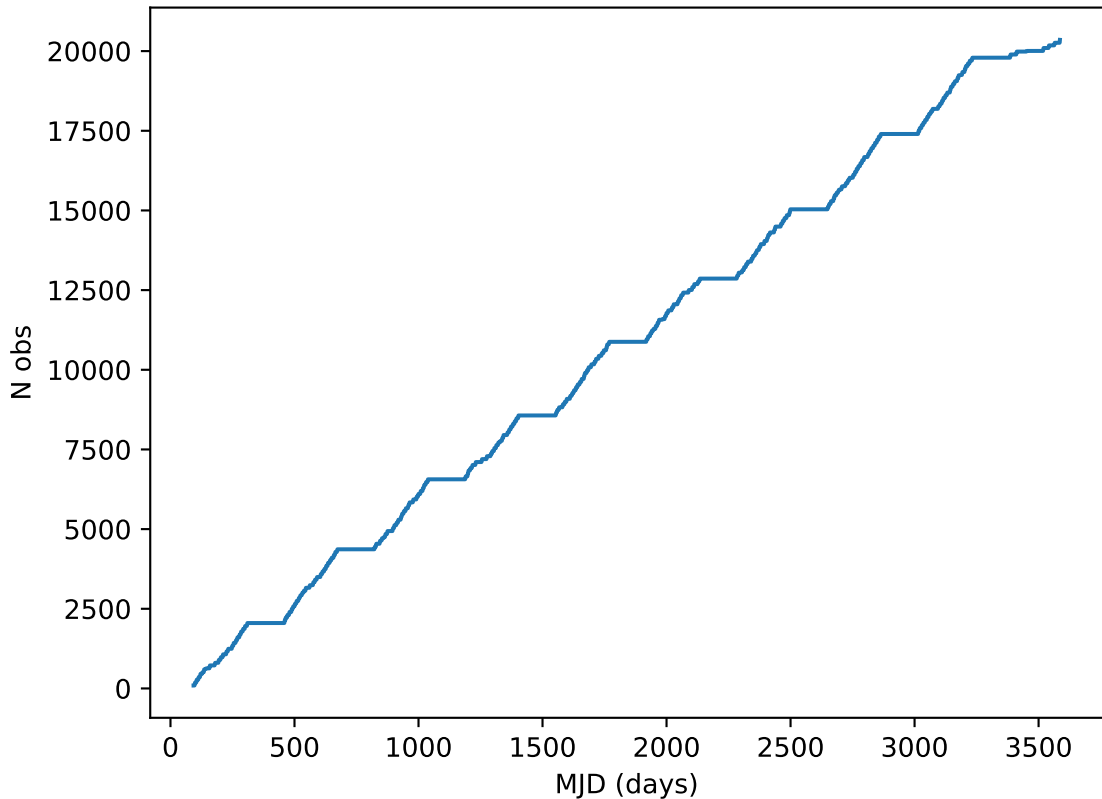
weather_cloudso35v3.4_10yrs all bands: DD:ECDFS Cumulative NVisits
