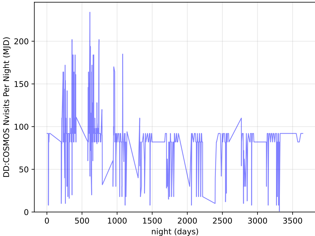
weather_cloudso35v3.4_10yrs all bands: DD: COSMOS Nvisits Per Night
