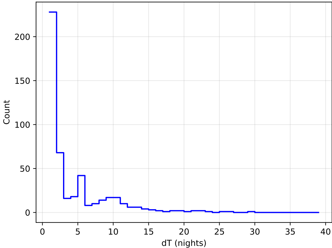
weather_cloudso35v3.4_10yrs all bands: DD: COSMOS Delta Nights Histogram
