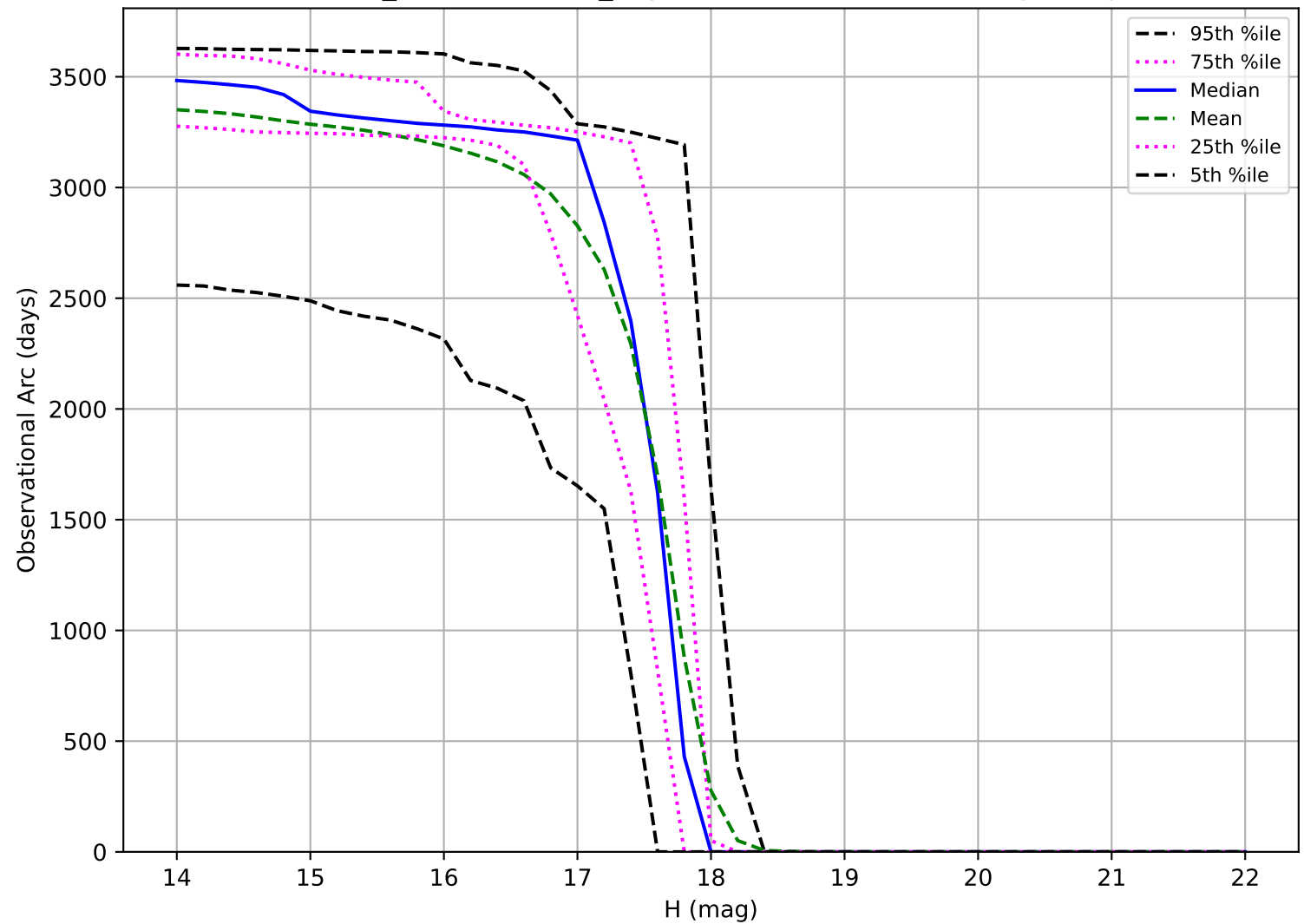
weather_cloudso31v3.4_10yrs: Observational Arc Length Trojan
