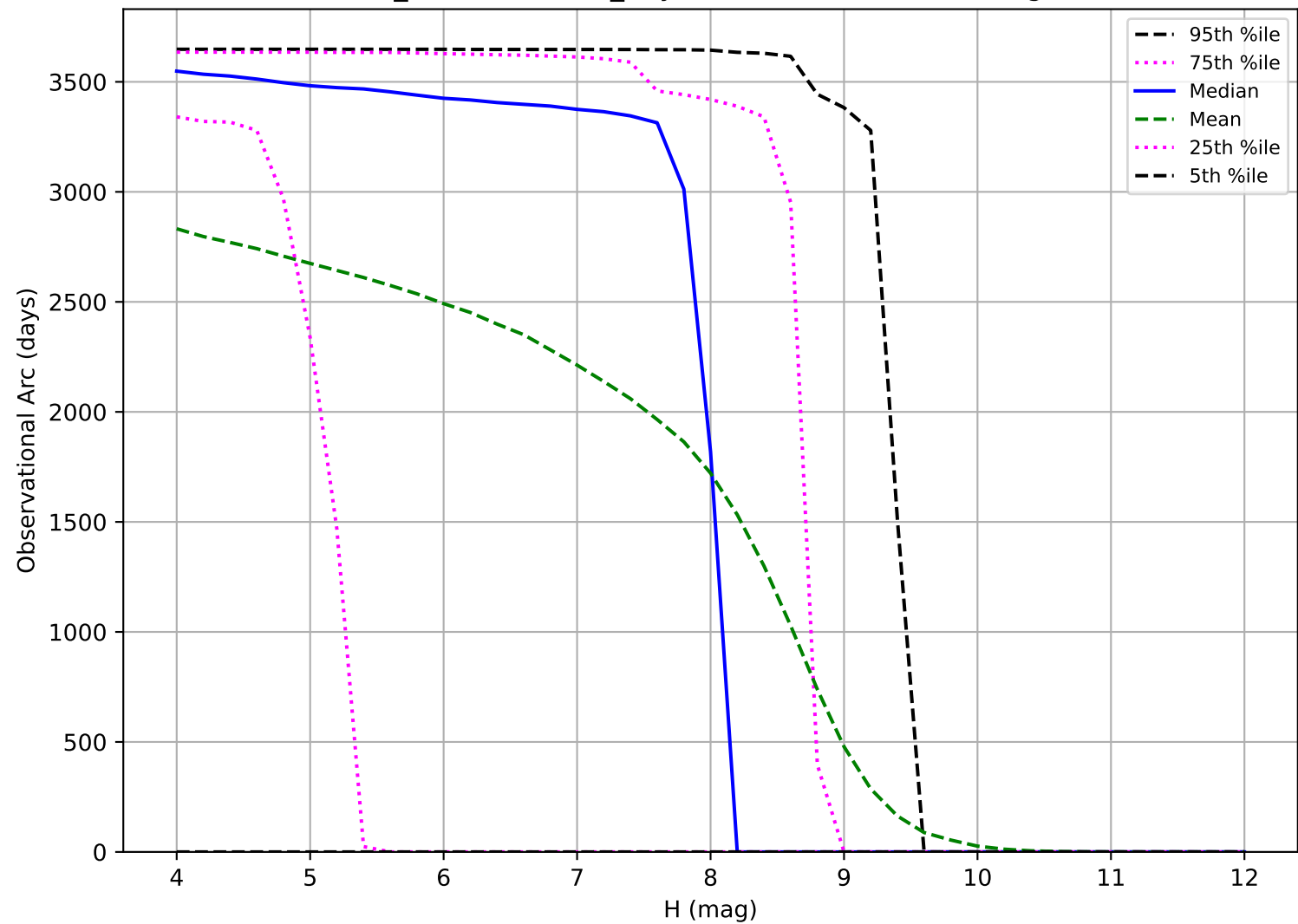
weather_cloudso31v3.4_10yrs: Observational Arc Length TNO
