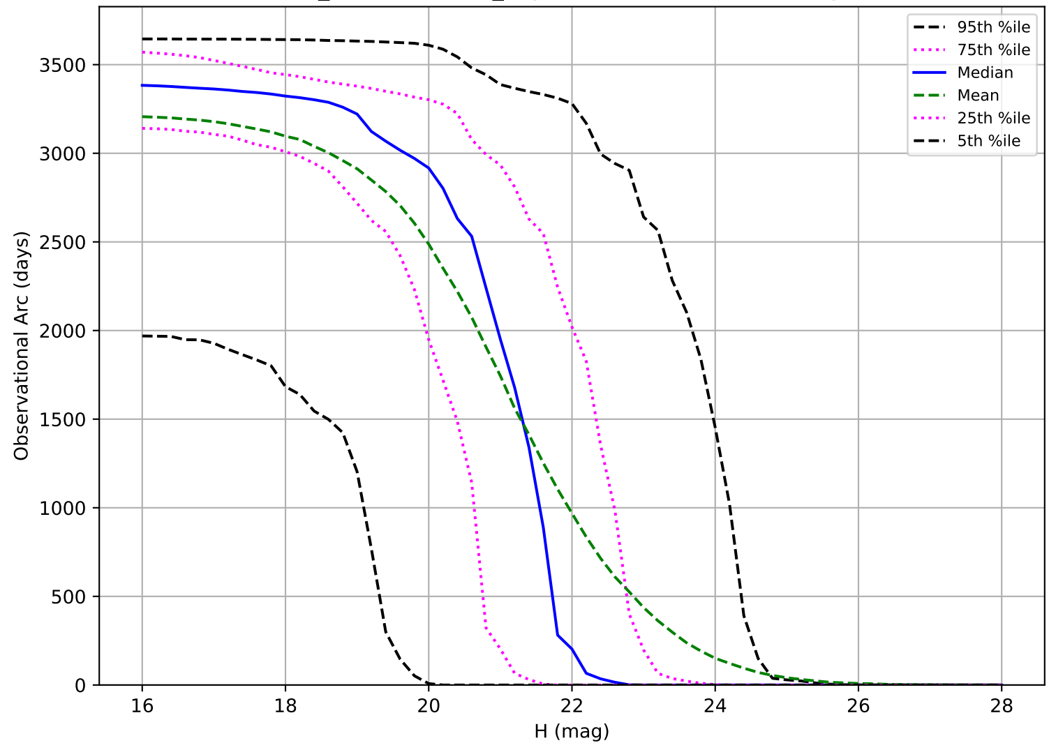
weather_cloudso31v3.4_10yrs: Observational Arc Length PHA
