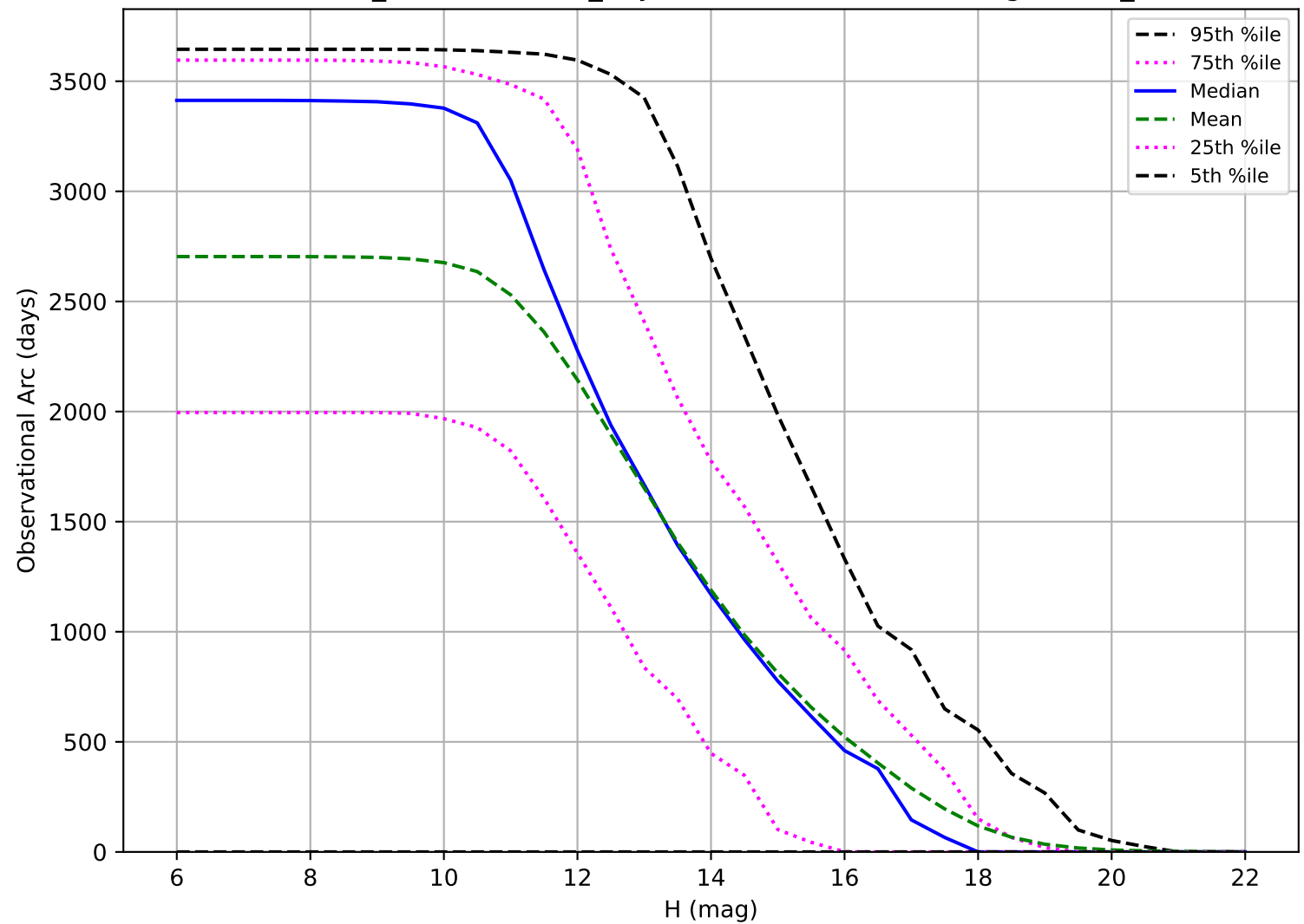
weather_cloudso31v3.4_10yrs: Observational Arc Length OCC_r5
