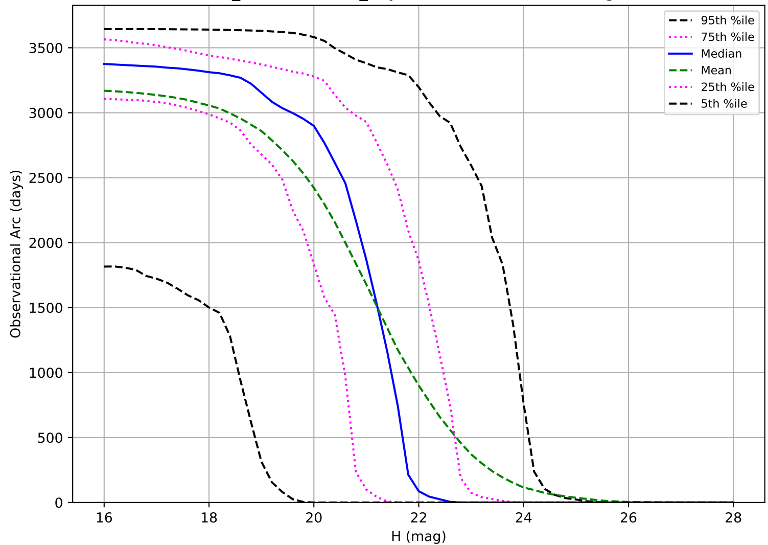
weather_cloudso31v3.4_10yrs: Observational Arc Length NEO
