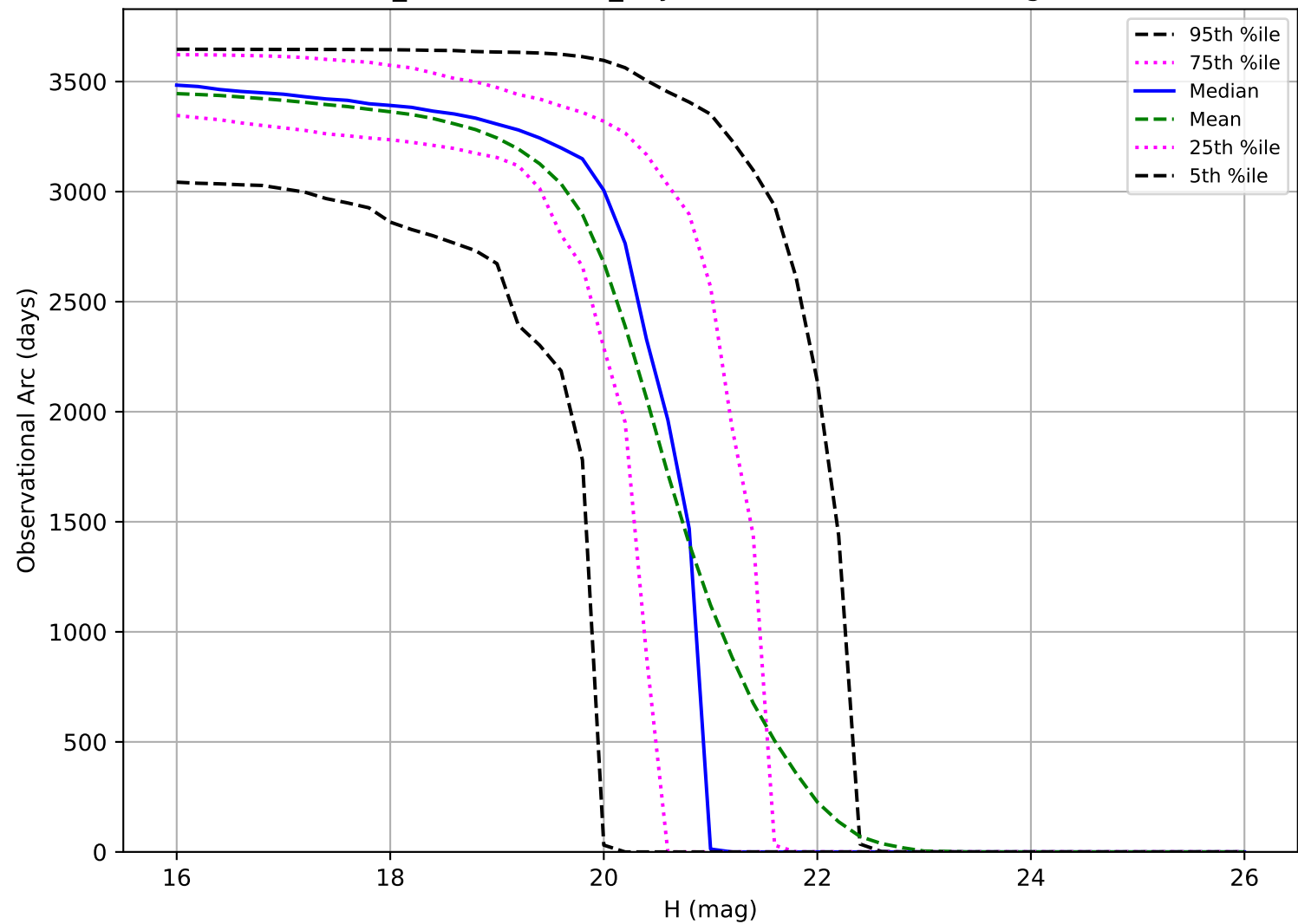
weather_cloudso31v3.4_10yrs: Observational Arc Length MBA
