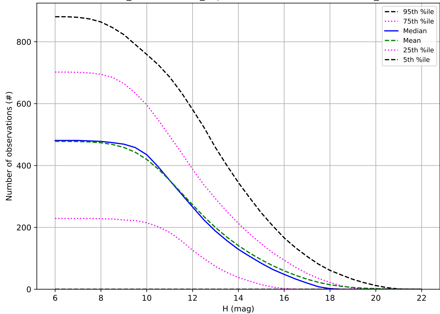
weather_cloudso31v3.4_10yrs: Number of observations OCC_r5
