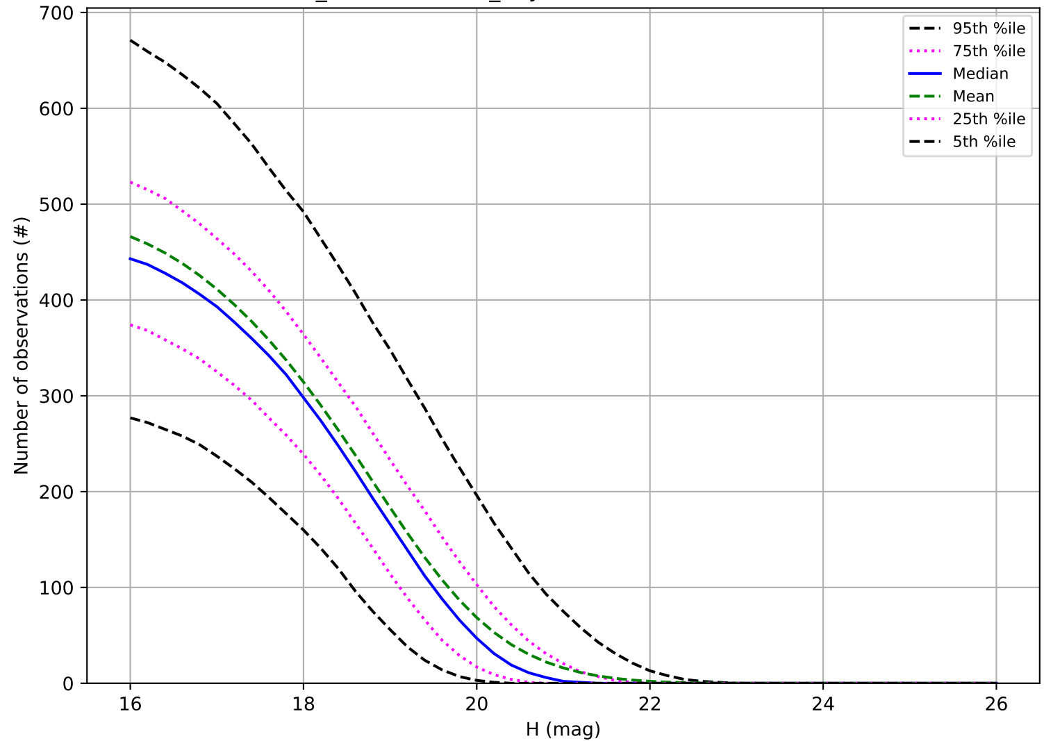
weather_cloudso31v3.4_10yrs: Number of observations MBA
