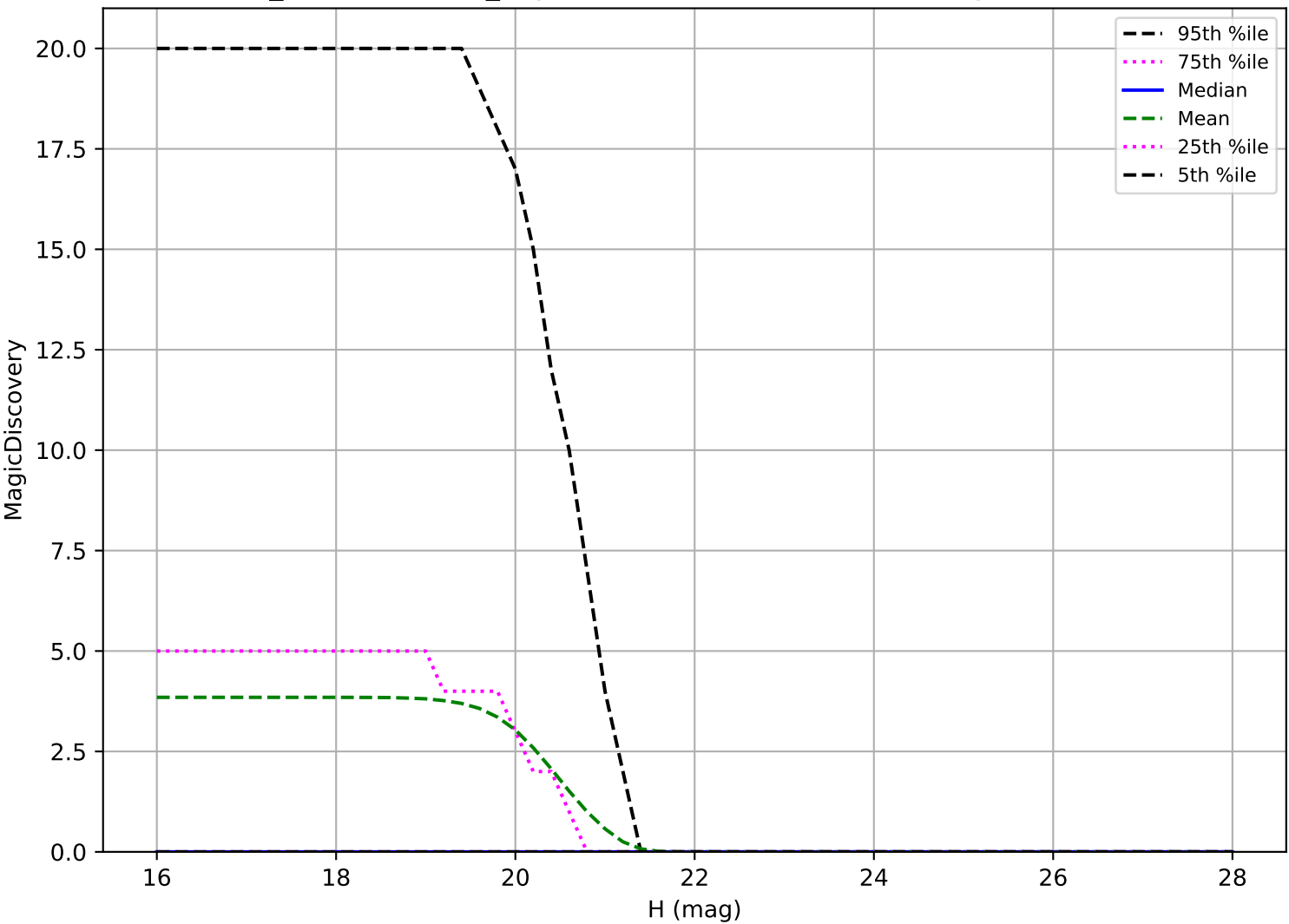
weather_cloudso31v3.4_10yrs: Vatira 6 detections in 60 nights detection loss
