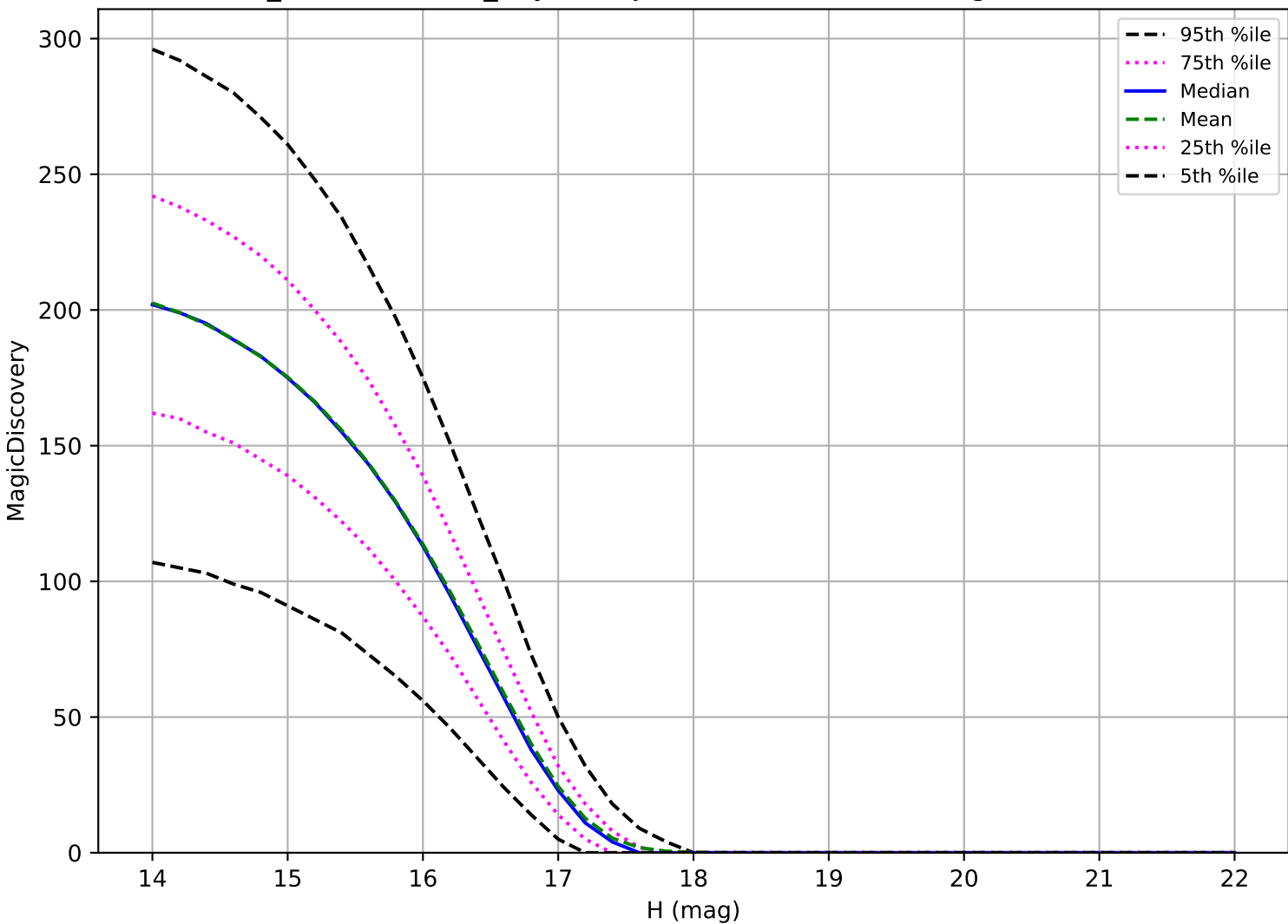
weather_cloudso31v3.4_10yrs: Trojan 6 detections in 60 nights detection loss
