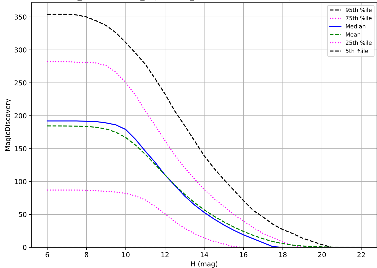
weather_cloudso31v3.4_10yrs: OCC_r5 6 detections in 60 nights detection loss
