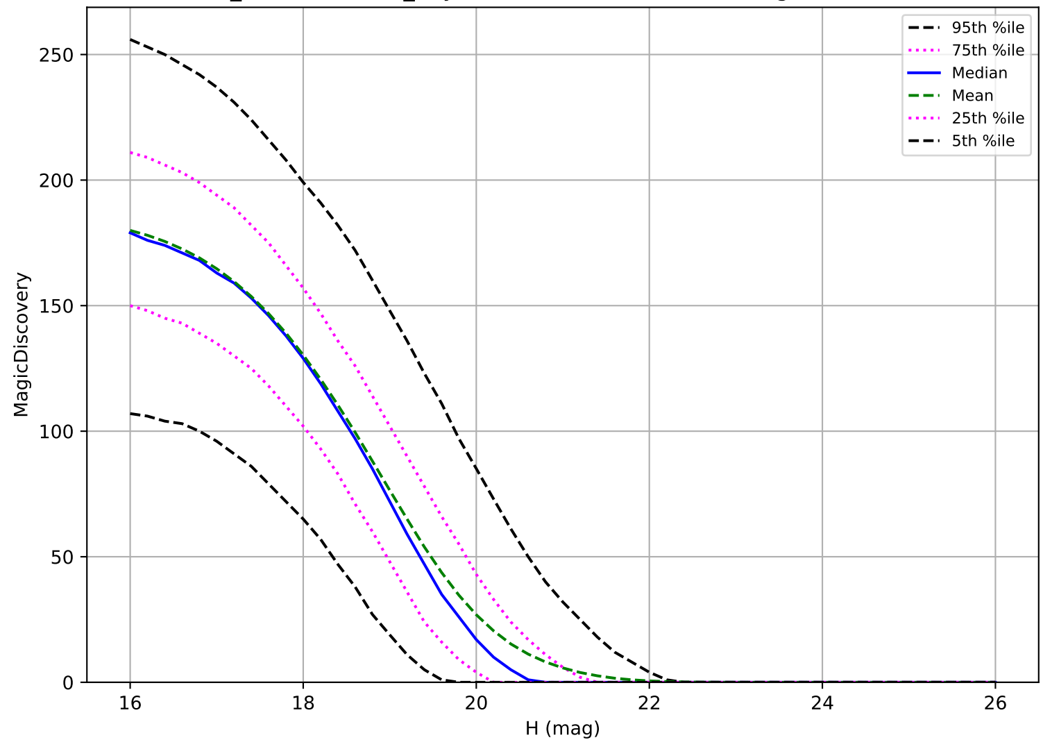
weather_cloudso31v3.4_10yrs: MBA 6 detections in 60 nights detection loss
