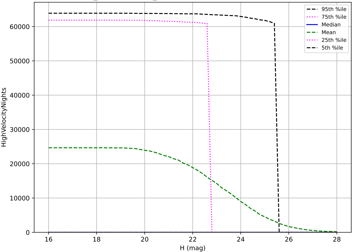
weather_cloudso31v3.4_10yrs: PHA High velocity pair detection loss
