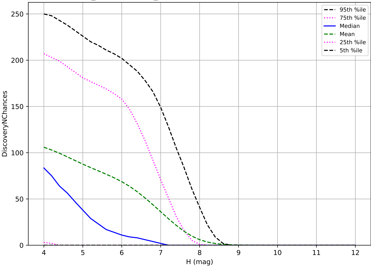
weather_cloudso31v3.4_10yrs: TNO 3 pairs in 15 nights detection loss
