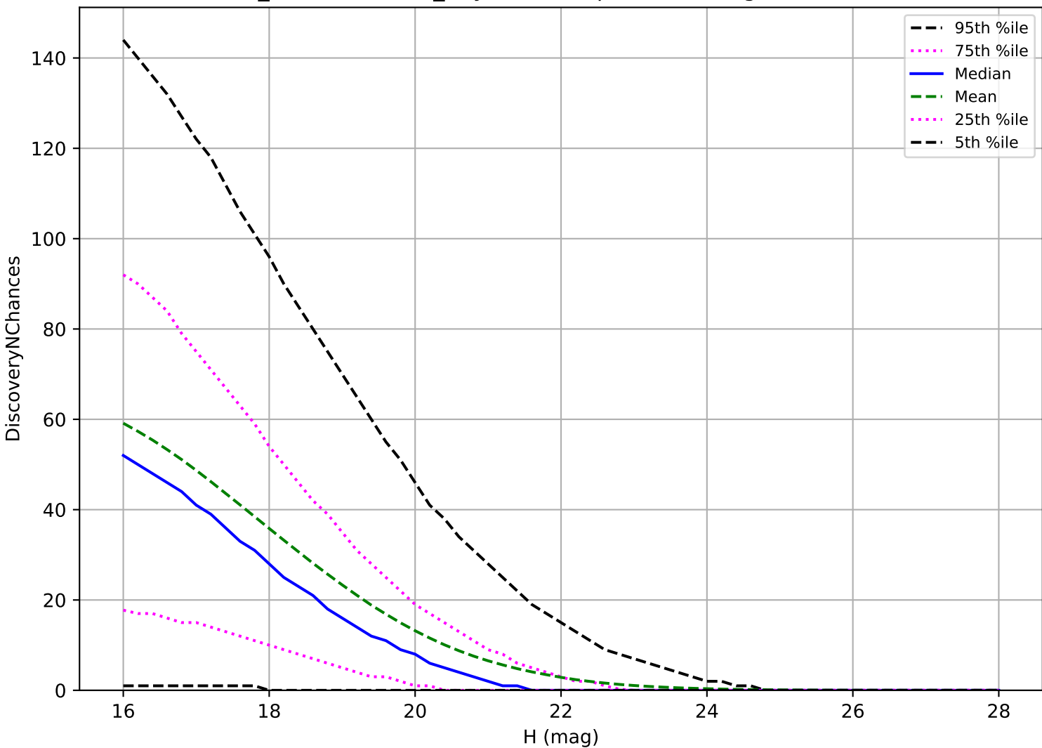
weather_cloudso31v3.4_10yrs: PHA 3 pairs in 15 nights detection loss
