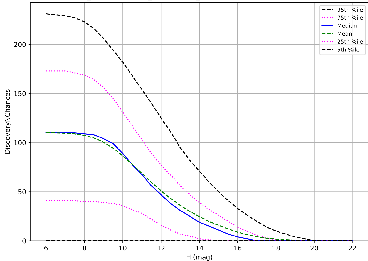
weather_cloudso31v3.4_10yrs: OCC_r5 3 pairs in 15 nights detection loss
