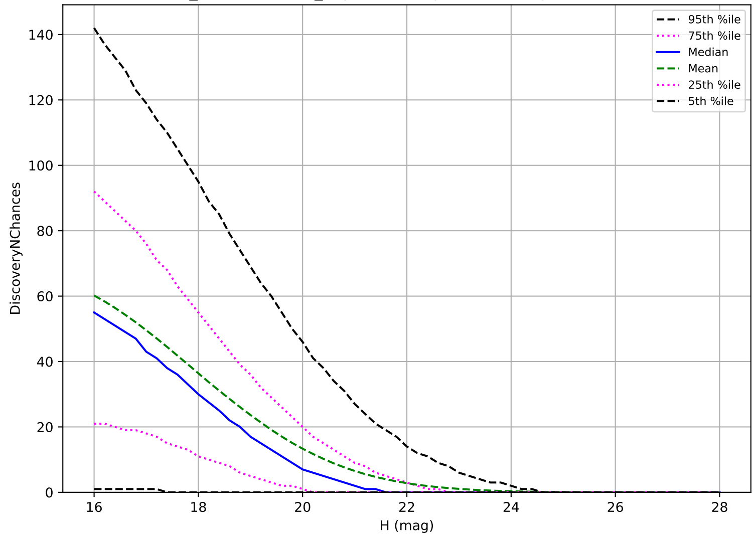
weather_cloudso31v3.4_10yrs: NEO 3 pairs in 15 nights detection loss
